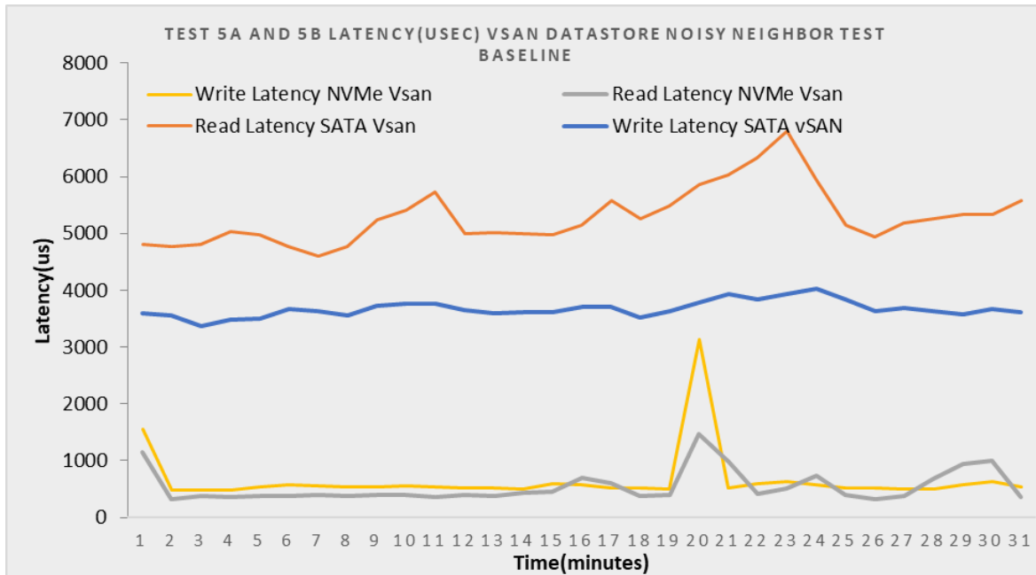
Figure 6.5 Test 5a and 5b Noisy Neighbor latency, DC1500M NVMe and Micron 5200 eco vSAN datastore
