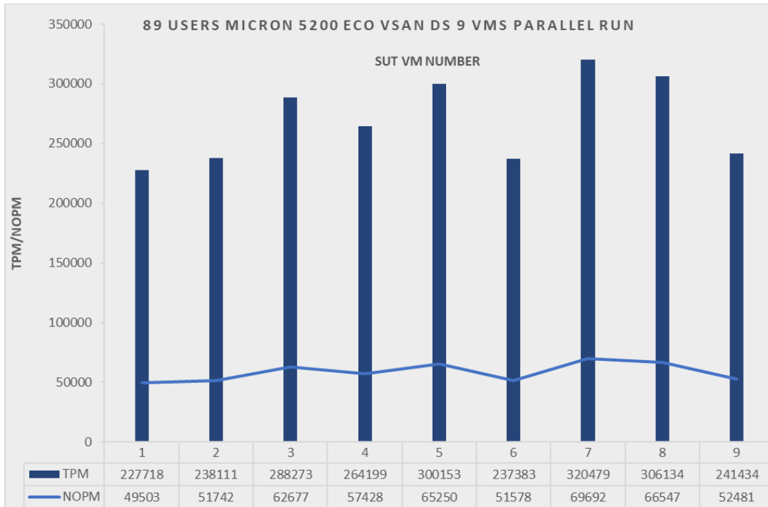
Figure 6.3 Test 5b TPM SQL Server 2017 300 min 12 VM parallel run, 89 virtual users, DC1500M NVMe SSD vSAN datastore
