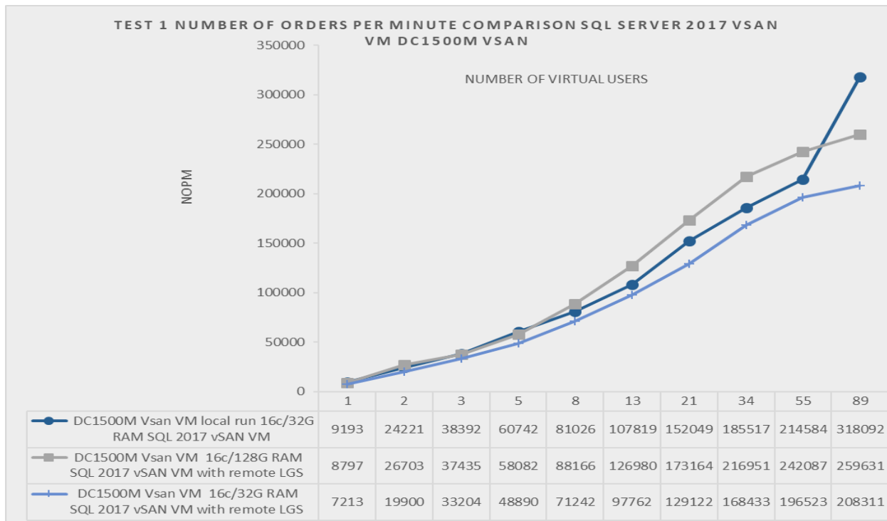
Figure 2.3 Test 1a,b,c: DC1500M vSAN datastore NOPM comparison different DRAM size
