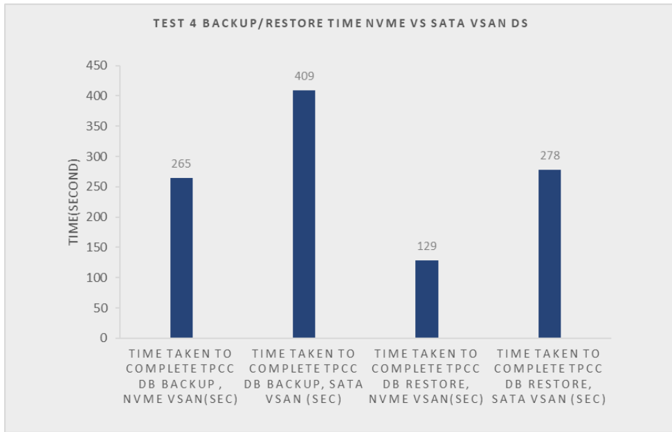
Figure 5.6 Time taken to complete SQL Server 2017 TPCC DB Backup/Restore operation Micron 5200 eco SATA and DC1500M NVMe SSD vSAN datastore(sec)
