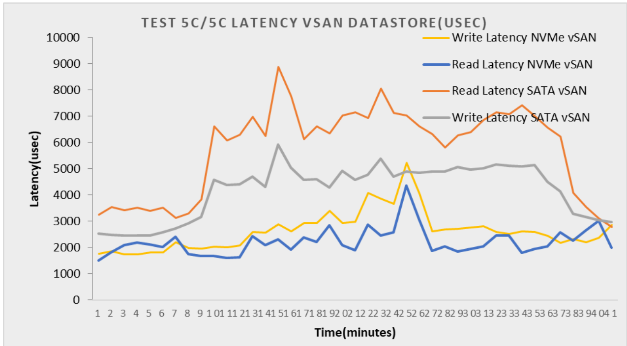
Figure 6.9 Test 5C/5D Latency, Noisy Neighbor implementation NVMe vs SATA SSD vSAN datastore
