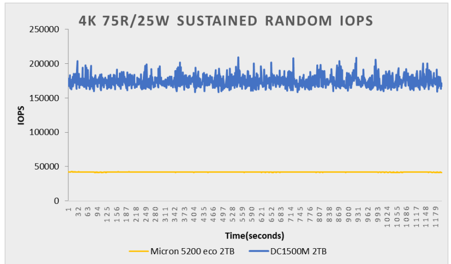
Figure a) Second-by-second IOPS comparison of DC1500M 1920G and Micron 5200 ECO 1920G SATA SSD. Tested on a single physical drive attached as a secondary to a linux system with fio v3.17 once the SSDs have reached a steady state of performance. Based on a block size of 4k, Read percentage of 75% and a Queue depth of 32
