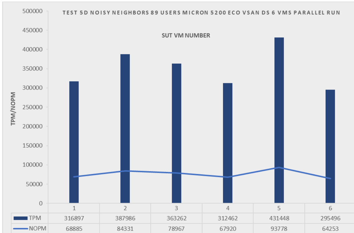
Figure 6.7 Test 5D TPM, Noisy Neighbor implementation 6 VM parallel run Micron 5200 eco vSAN datastore
