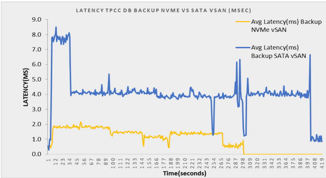
Figure 5.3 Avg Latency(ms) comparison SQL Server 2017 TPCC DB Backup Micron 5200 eco SATA and DC1500M NVMe SSD vSAN datastore
