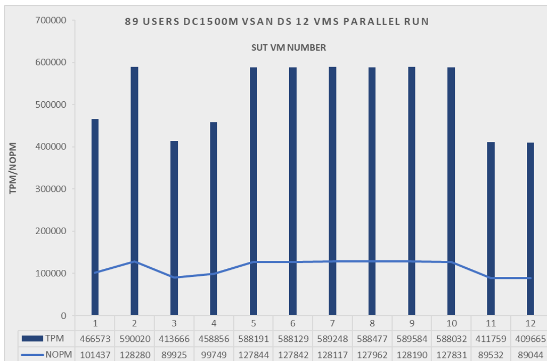
Figure 6.2 Test 5a TPM SQL Server 2017 300 min 12 VM parallel run, 89 virtual users, DC1500M NVMe SSD vSAN datastore
