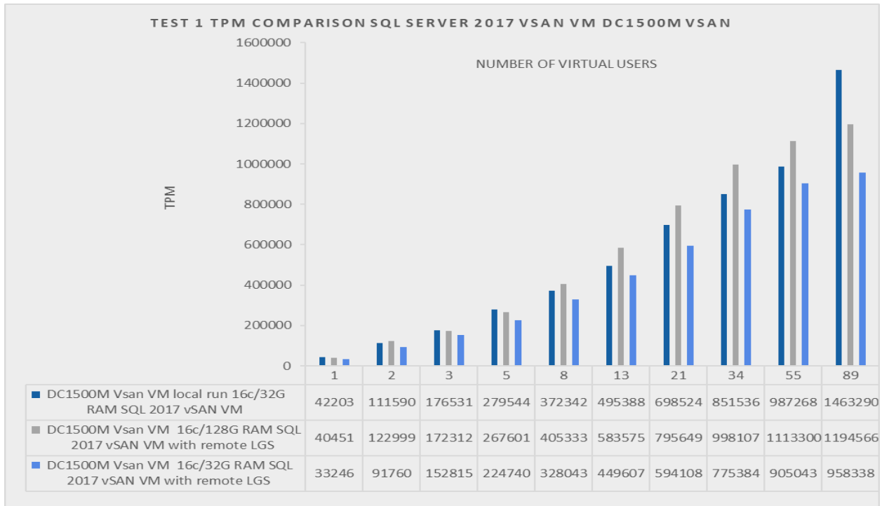
Figure 2.2 Test 1a,b,c: DC1500M vSAN datastore TPM comparison different DRAM size
