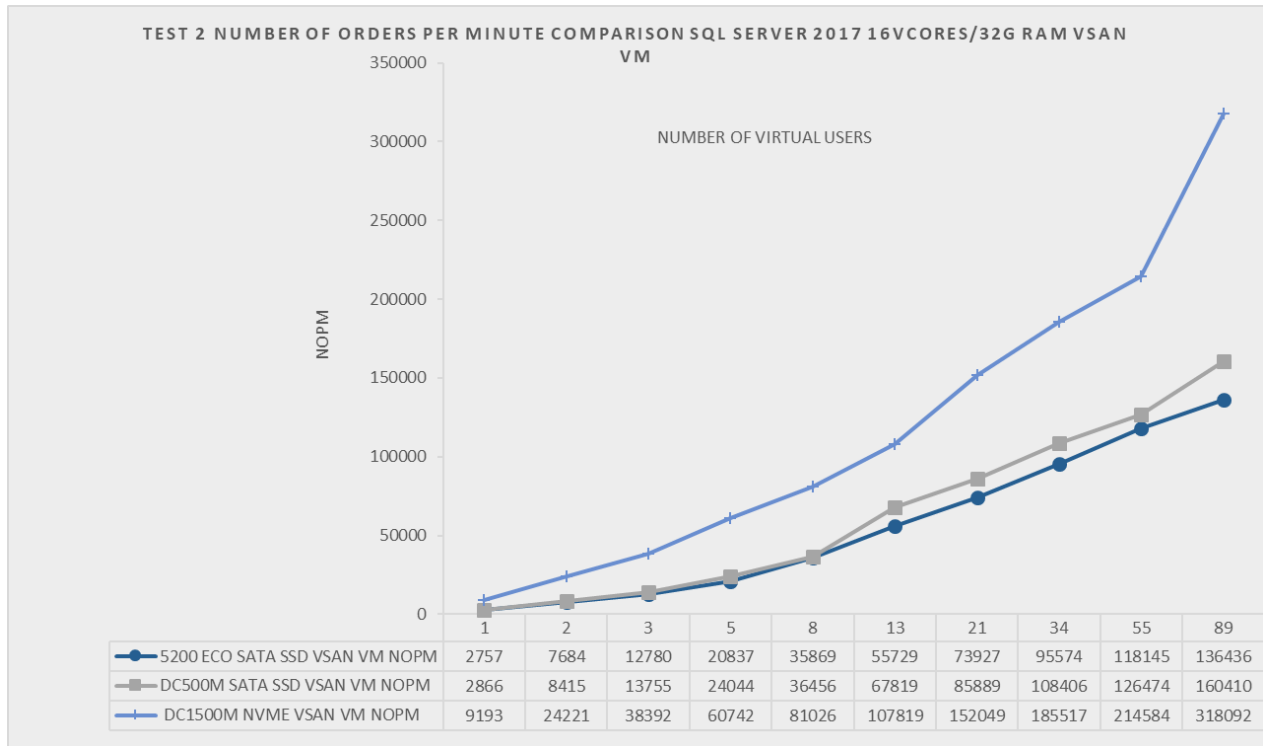
Figure 3.3 Test 2: NOPM comparison NVME VS SATA VSAN datastore
