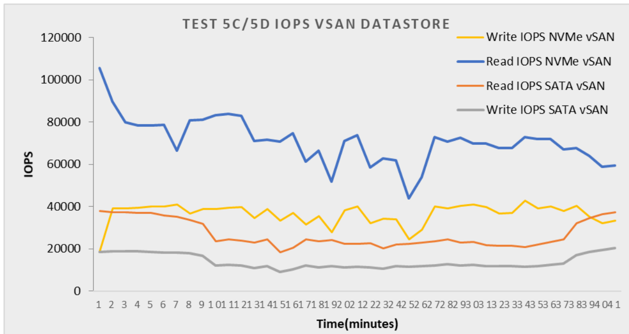
Figure 6.8 Test 5C/5D IOPS, Noisy Neighbor implementation NVMe vs SATA SSD vSAN datastore
