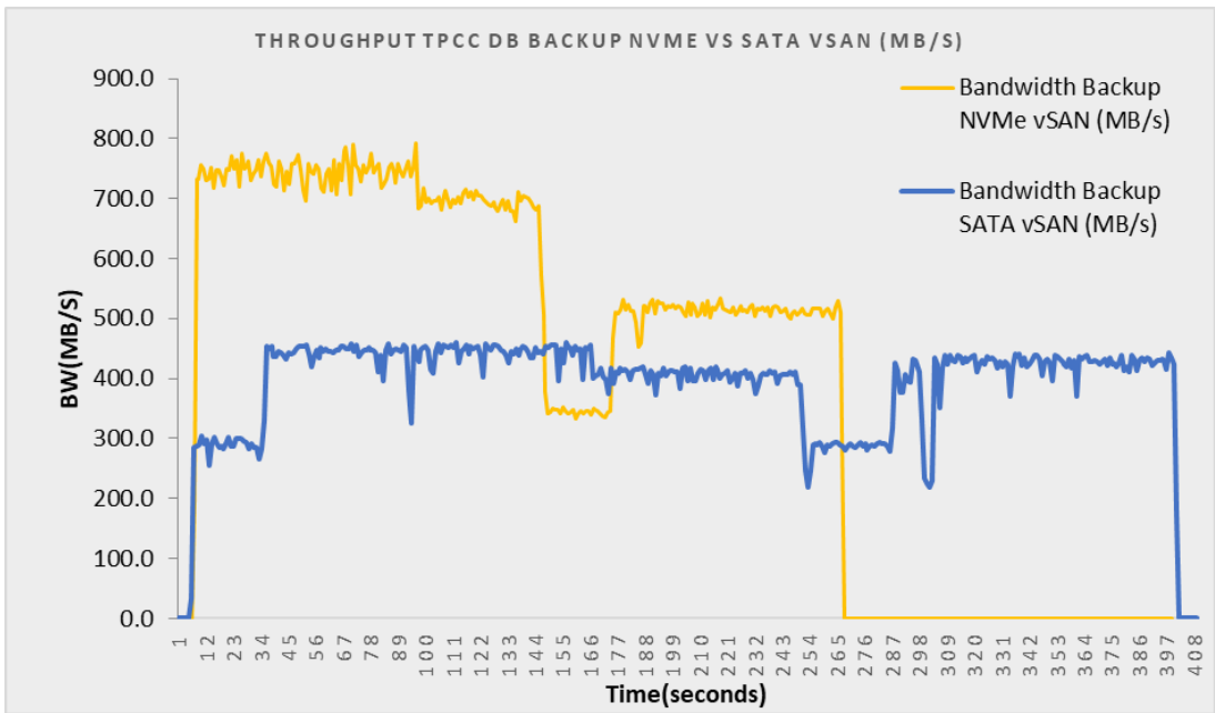
Figure 5.2 Throughput comparison SQL Server 2017 TPCC DB Backup Micron 5200 eco SATA and DC1500M NVMe SSD vSAN datastore(MB/s)
