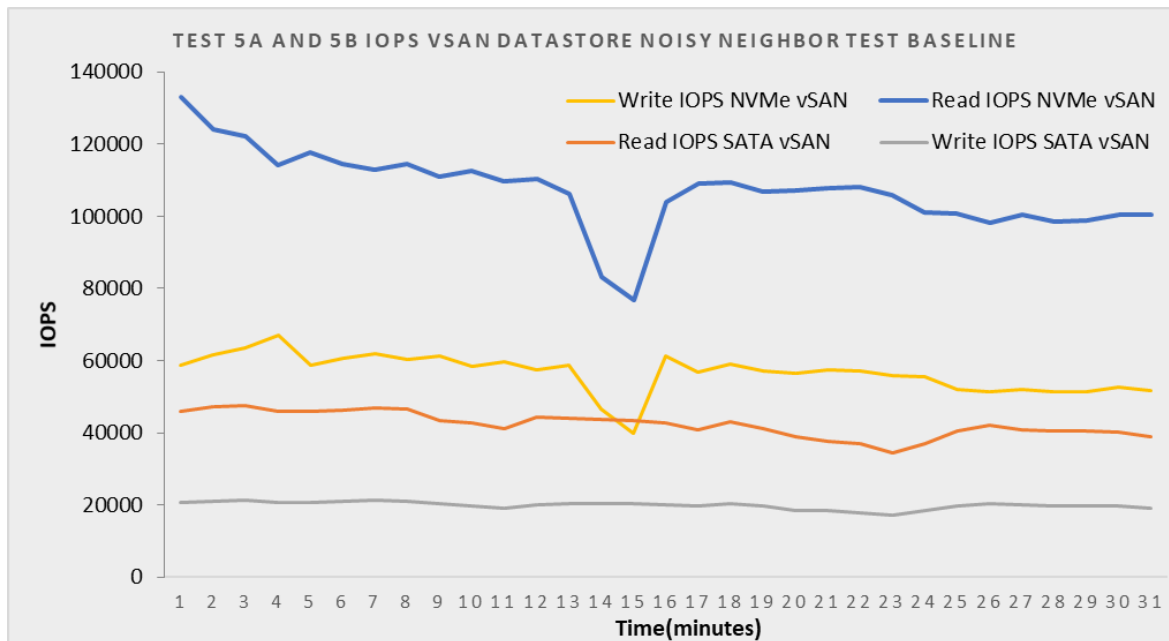
Figure 6.4 Test 5a and 5b Noisy Neighbor IOPS, DC1500M NVMe and Micron 5200 eco vSAN datastore
