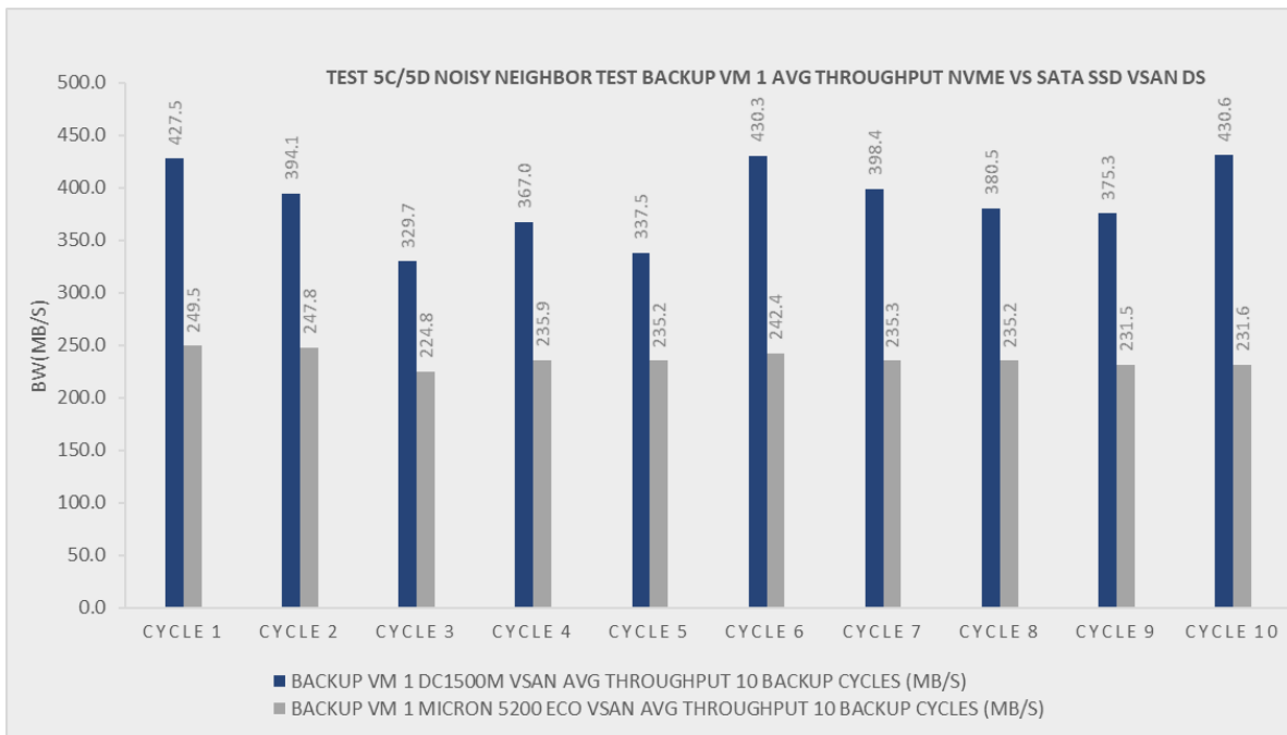
Figure 6.10 Test 5C/5D Backup VM throughput, Noisy Neighbor implementation NVMe vs SATA SSD vSAN datastore
