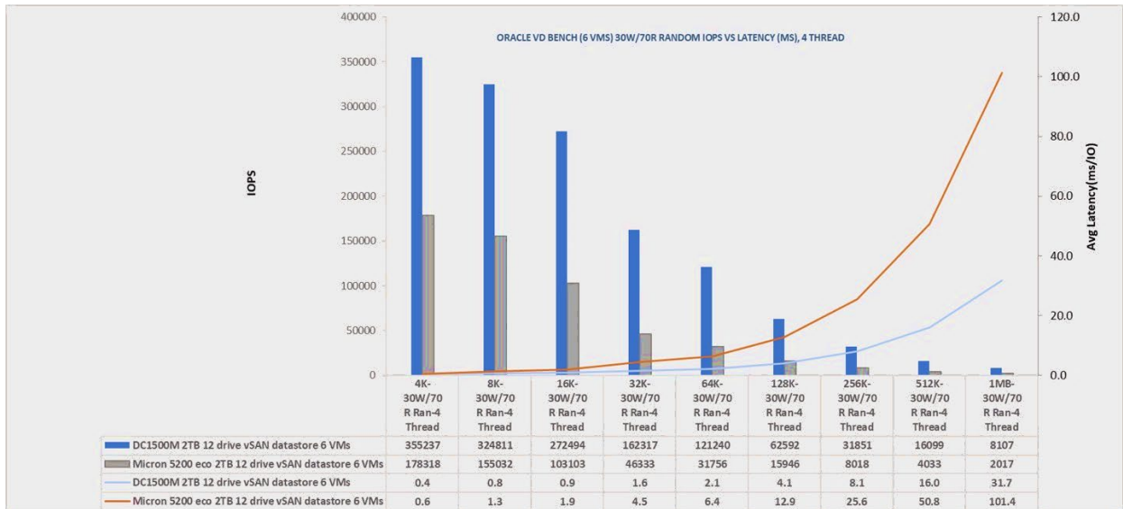
Figure 1.3 DC1500M vSAN datastore vs Micron 5200 eco vSAN datastore, 4k 70R/30W, Random, QD=8, threads=4, 6 VMs HCIBench IOPS vs average latency(ms)
