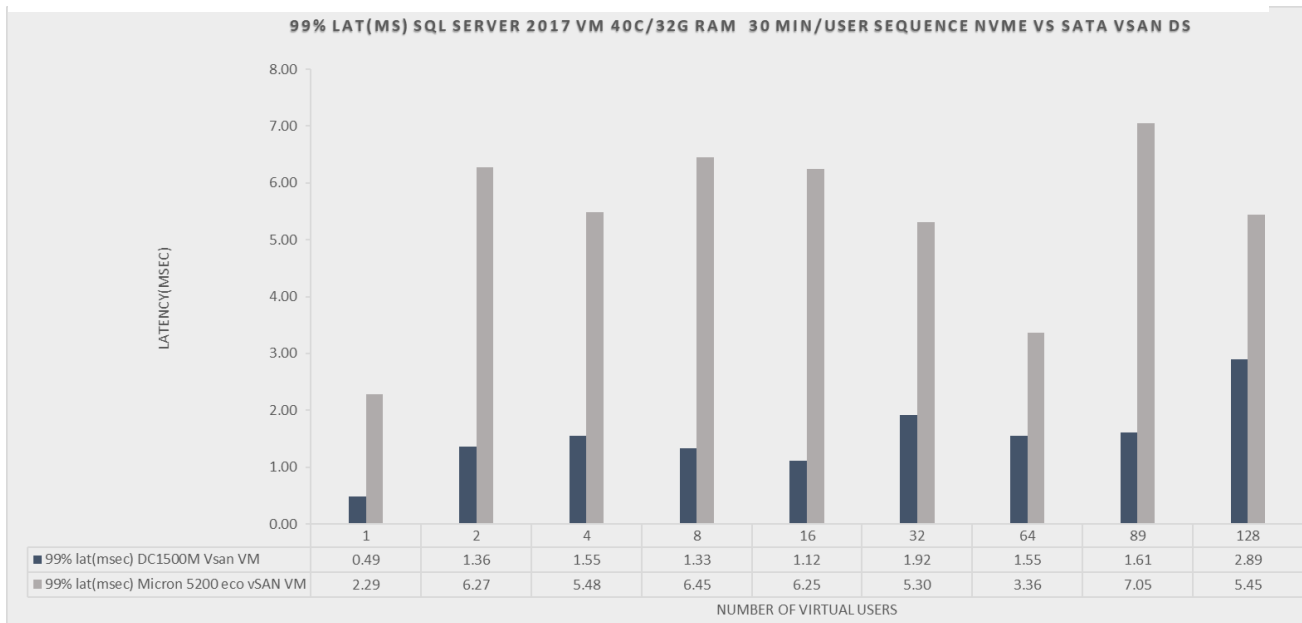
Figure 4.5 Test 3 99 th % Latency(ms) comparison SQL Server 2017 DB stress test on Micron 5200 eco SATA and DC1500M NVMe SSD vSAN datastore
