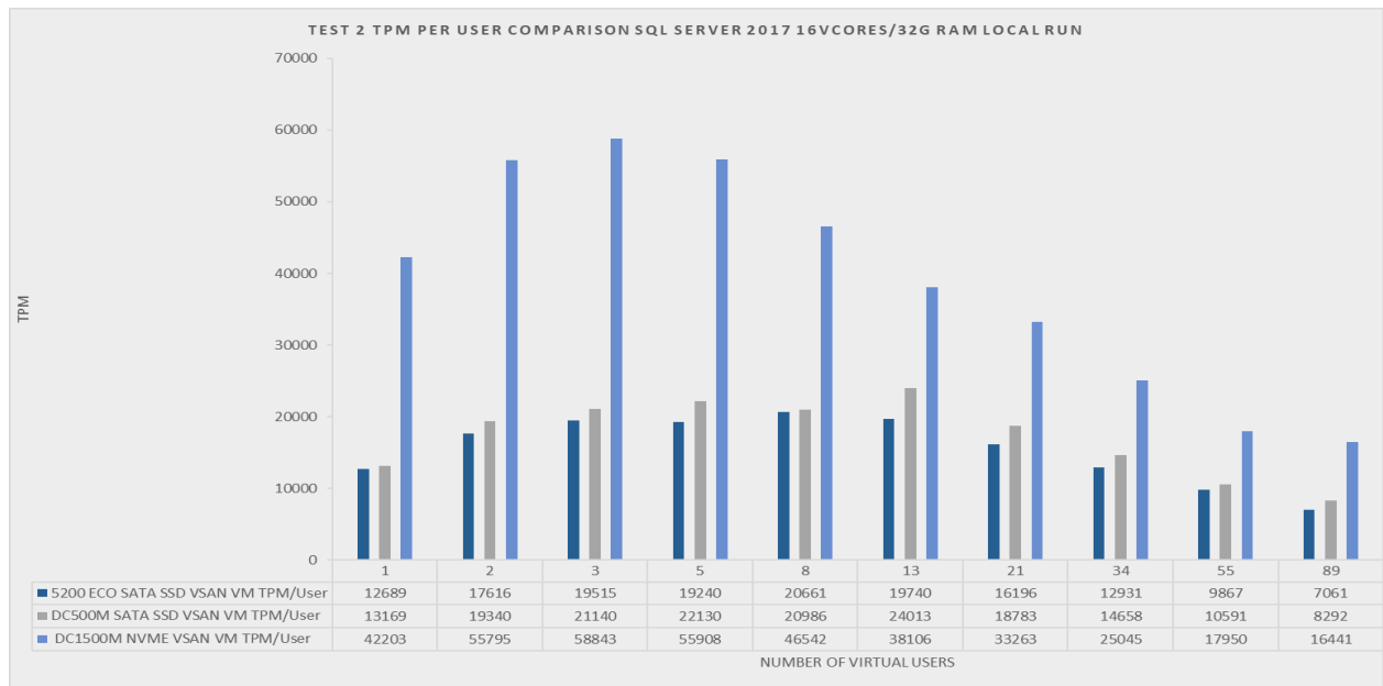
Figure 3.4 Test 2: TPM per user comparison NVME VS SATA VSAN datastore
