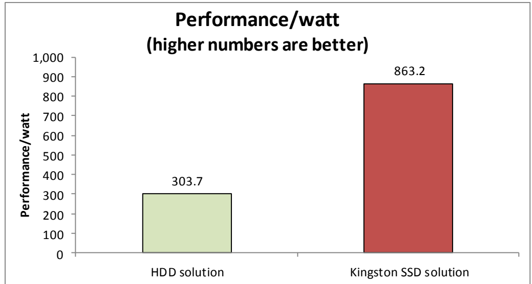
Figure 2: Performance/watt for the two solutions.
