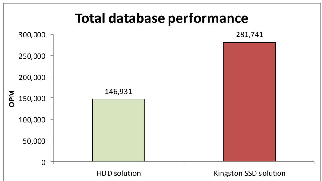
Figure 1: Using six Kingston SSDs increased performance over an all-HDD (24 drives) solution by 91.8 percent.
