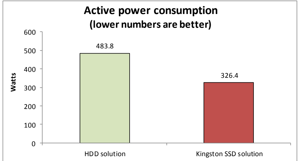
Figure 3: Power, in watts, that the solutions consumed while running database workloads.
